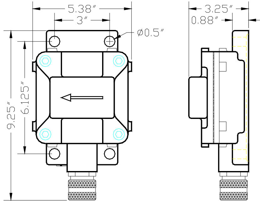
SWITCH MSW-L
